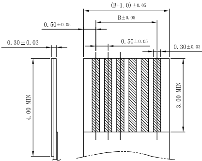
RECOMMENDED FPC/FFC DIMENSION
